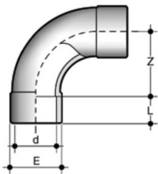
SIV 90° long radius bend (R=2d) with solvent weld sockets
